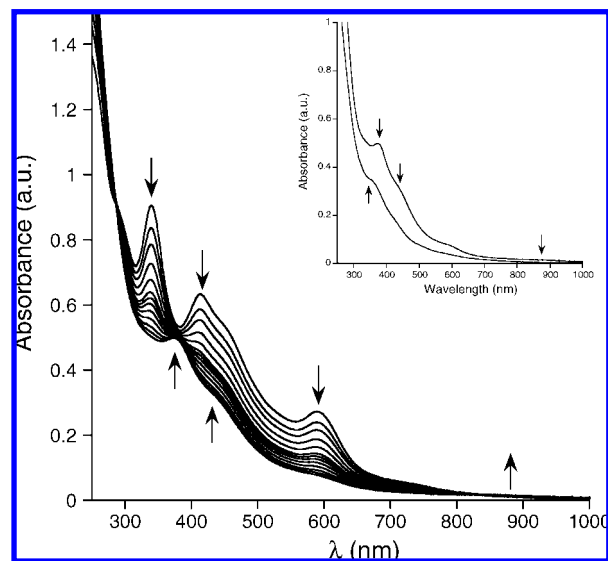
Figure 2. UV–vis spectrum of the reaction of (^t\text{Bu}_4\text{N})_2[\text{Fe}_2\text{S}_2(\text{S}_2\text{-}o\text{-xyl})_2] (64 \mu\text{M} ) with excess ( \sim 30 equiv) \text{NO}(\text{g}) at 298 K in MeCN. Spectra were recorded over 45 min. Inset shows the spectral change associated with transformation of the DNIC to RBS.
