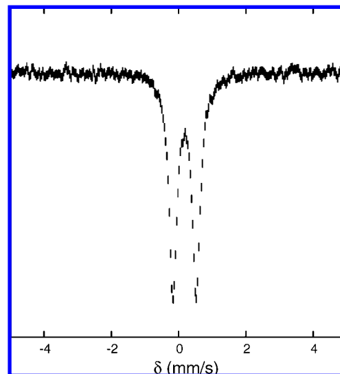
Figure 4. Zero-field Mössbauer (4.2 K) spectrum of (\text{Et}_4\text{N})[\text{Fe}(\text{NO})_2(\text{SPh})_2] . See Supporting Information (Figure S5) for the theoretical fit from which the isomer shift and quadrupole splitting parameters were obtained.
